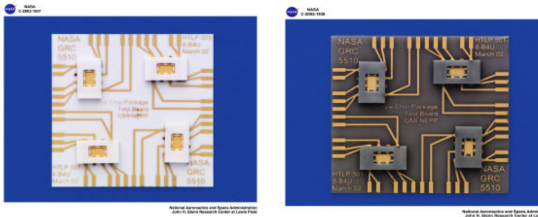
Figure 3: Aluminum oxide and aluminum nitride high temperature 8-pin chip level packages and printed circuit boards.
