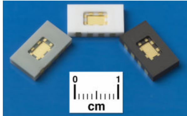
Figure 2: AlN and Al 2 O 3 based chip level packages for SiC devices.
