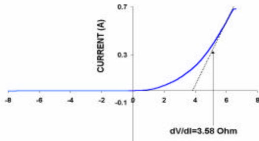
Figure 1: I-V curve of a SiC Schottky diode measured in 500°C oxidizing environment after 1000 hrs at 500°C.
