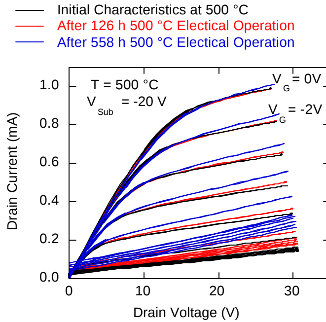
Figure 4: I-V curves of packaged SiC MESFET at various gate biases for V_{\text{Sub}} = -20\text{ V} .
