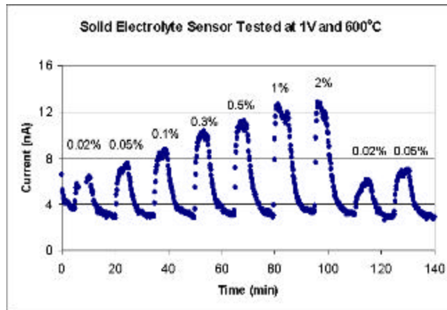
Figure 6: Response of a NASICON based CO 2 sensor tested at 1 volt, 600 °C to varying CO 2 concentration: .02%, 0.05%, 0.1%, 0.3%, 0.5%, 1%, and 2%.
