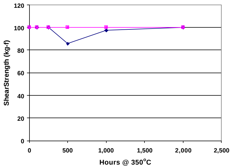
Figure 9: Die shear of 3.8mm x 3.8 mm die after storage at 350°C with the AuSn braze, AuIn was used as a base line (measured by Prof. Johnson's group at Auburn University).
