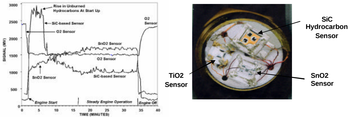
Figure 5: a) The response of a packaged sensor array composed of a tin oxide based sensor (doped for \text{NO}_x sensitivity), an oxygen sensor, and a SiC-based hydrocarbon sensor in an engine environment. b) Optical micrograph of high temperature SiC Schottky diode and metal thin film resistive sensors in a ceramic package.
